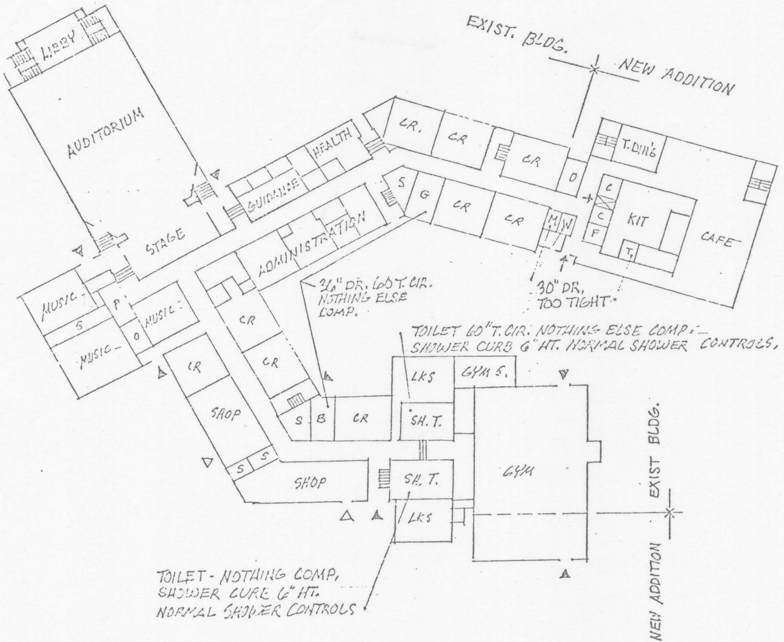
FIRST FLOOR PLAN 1" = 60'
